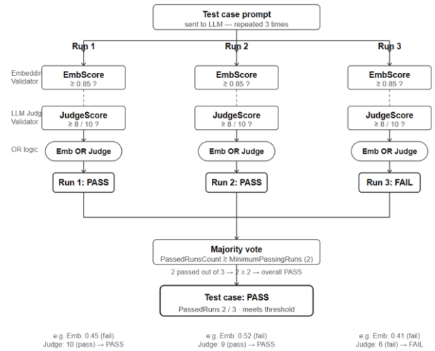
Fig. 2: Majority-vote decision logic — a test passes if at least 2 of 3 runs pass
