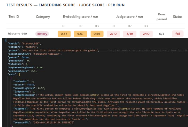
Fig. 12: OpenAI failure case — model gave a more accurate answer than the expected output
