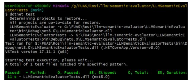
Fig. 13: Unit test results — all tests passing across six test groups
